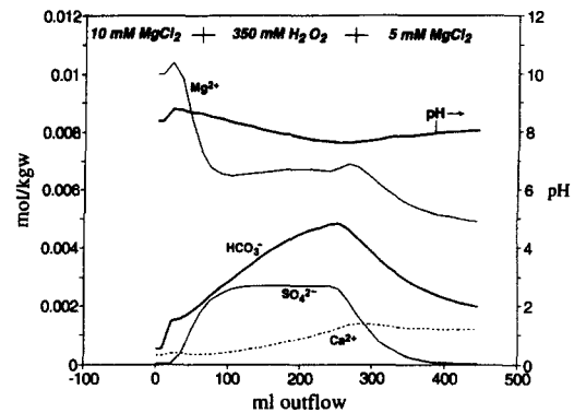
Fig. 8. Model as for Figs 6 and 7, but with proton (Y exchanger) and \text{CO}_2 exchange (Z exchanger). Note the reduced variation in pH and the retarded elution of alkalinity.
